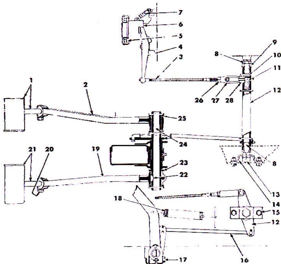
FIG. 174—CLUTCH CONTROL—MODELS CJ-2A, CJ-3A AND DJ-3A
